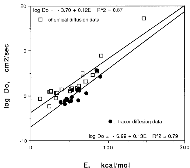
Fig. 4. Compensation law plot of the Arrhenius frequency factor, \log_{10} D_0 , against the Arrhenius activation energy, E , for all known oxygen diffusion measurements in silicate melts (modified from Schreiber et al. 1986). Solid lines are least-squares fits. Chemical diffusion data (24 measurements) includes results of this study, Doremus (1960), Lawless and Wedding (1970), Sasabe and Goto (1974), Dunn (1983), Semkow and Haskin (1985), and Schreiber et al. (1986). Tracer diffusion data (17 measurements) include results of Koros and King (1962), May et al. (1974), Muehlenbachs and Kushiro (1974), Oishi et al. (1975), deBerg and Lauder (1978, 1980), Yinnon and Cooper (1980), Dunn (1982), Schaeffer et al. (1983), Shimizu and Kushiro (1984), and Canil and Muehlenbachs (1990)
