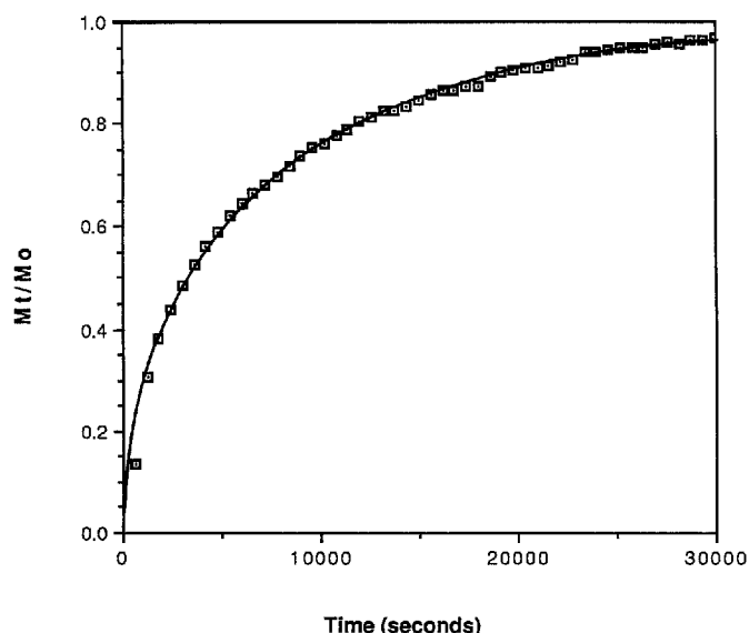
Fig. 1. Experimental measurements (squares) showing change in fractional saturation, M_t/M_o , of Goose Island basalt as a function of elapsed time (experiment 9; 1160° C). The solid line represents the calculated oxygen chemical diffusivity. Data were collected at 10 min intervals. The total weight change is approximately 1.5 mg
